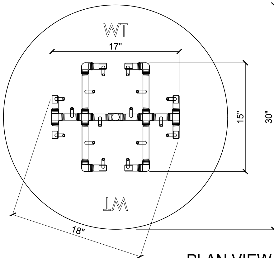
PLAN VIEW
