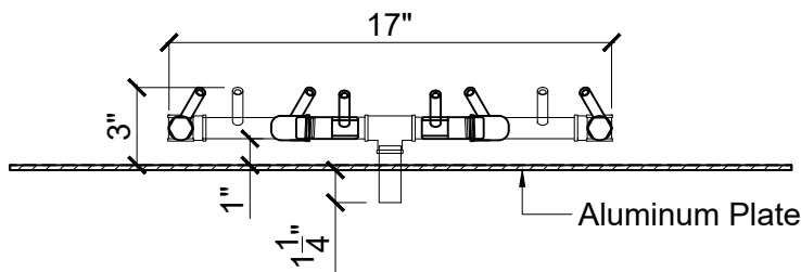
ELEVATION VIEW
